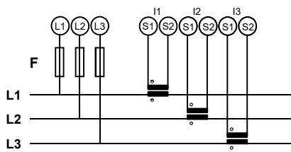
Three-phase, 3-wire, connection with 3 CTs
