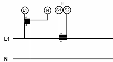
Single-phase, 2-wire, connection with 1 CT and 1 VT
