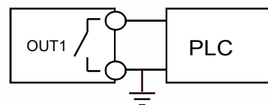
Digital output
