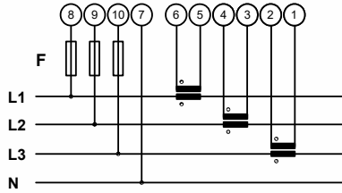
Three-phase, 4-wire, connection with 3 CTs
